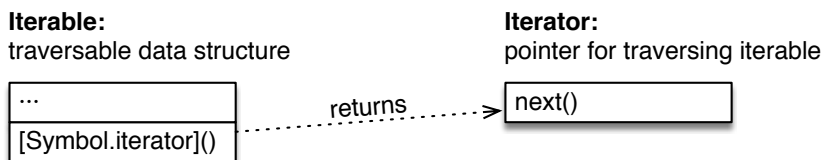
Figure 30.2: Iteration has two main interfaces: Iterable and Iterator . The former has a method that returns the latter.
