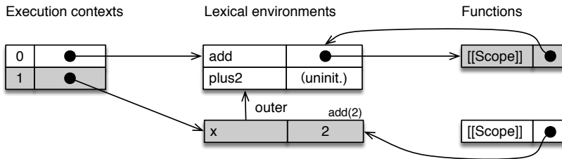
Figure 26.7: Closures, pause 1 – during the execution of add(2) : We can see that the function returned by add() already exists (see bottom right corner) and that it points to its birth environment via its internal property [[Scope]] . Note that plus2 is still in its temporal dead zone and uninitialized.
