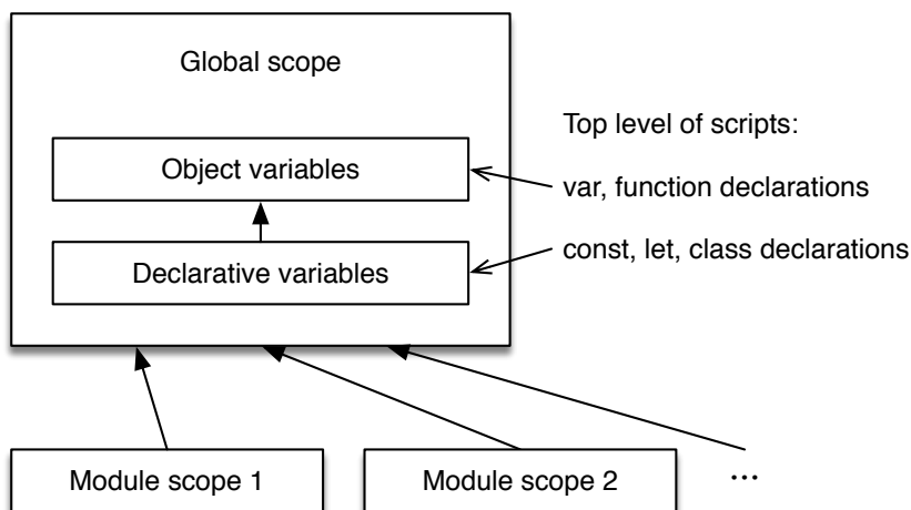
Figure 12.1: The global scope is JavaScript’s outermost scope. It has two kinds of variables: object variables (managed via the global object ) and normal declarative variables . Each ECMAScript module has its own scope which is contained in the global scope.
