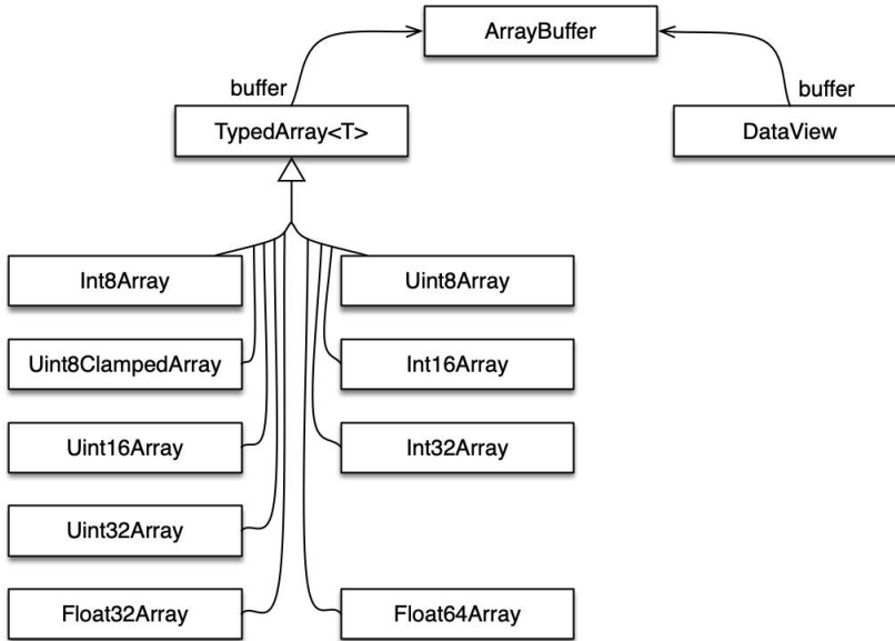
Figure 32.1: The classes of the Typed Array API.
