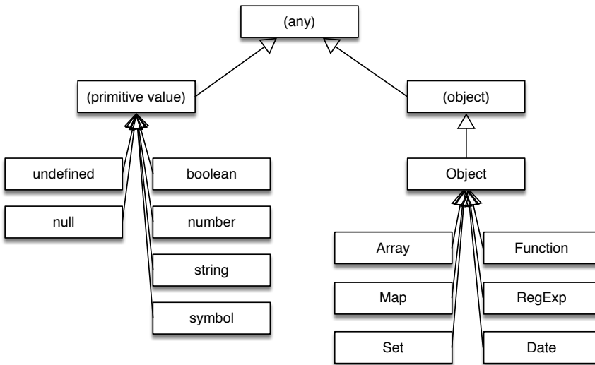
Figure 13.1: A partial hierarchy of JavaScript's types. Missing are the classes for errors, the classes associated with primitive types, and more. The diagram hints at the fact that not all objects are instances of Object .
