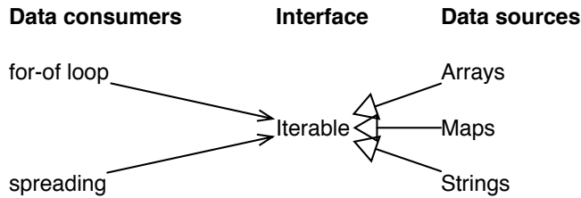
Figure 30.1: Data consumers such as the for-of loop use the interface Iterable . Data sources such as Arrays implement that interface.
