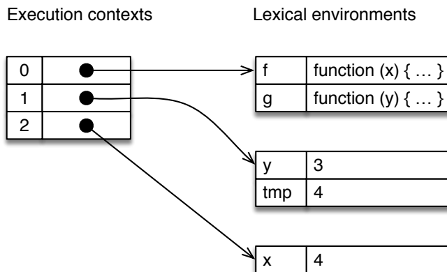
Figure 26.3: Recursion, pause 3 – while executing f() : The top execution context now points to the environment for f() .
