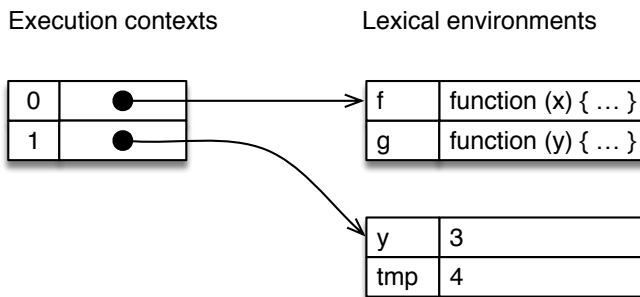
Figure 26.2: Recursion, pause 2 – while executing g() : The top of the execution context stack points to the environment that was created for g() . That environment contains entries for the argument y and for the local variable tmp .
