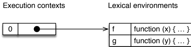
Figure 26.1: Recursion, pause 1 – before calling g() : The execution context stack has one entry, which points to the top-level environment. In that environment, there are two entries; one for f() and one for g() .
