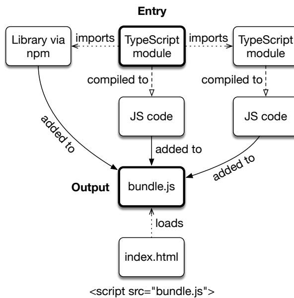
Figure 46.2: This is the workflow when developing a web app with the bundler webpack . Our web app consists of multiple modules. We tell webpack , in which one execution starts (the so-called entry point ). It then analyzes the imports of the entry point, the imports of the imports, etc., to determine what code is needed to run the app. All of that code is put into a single script file.
