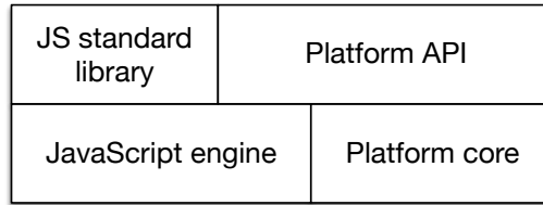
Figure 7.1: The structure of the two JavaScript platforms web browser and Node.js . The APIs “standard library” and “platform API” are hosted on top of a foundational layer with a JavaScript engine and a platform-specific “core”.
