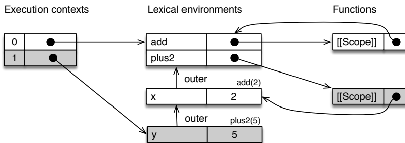
Figure 26.9: Closures, pause 3 – while executing plus2(5) : The [[Scope]] of plus2 is used to set up the outer of the new environment. That's how the current function gets access to x .
