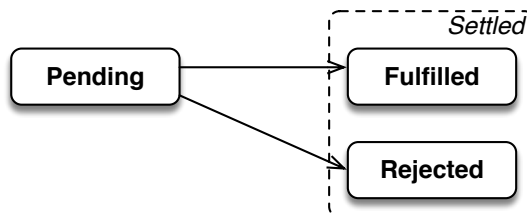
Figure 40.1: A Promise can be in either one of three states: pending, fulfilled, or rejected. If a Promise is in a final (non-pending) state, it is called settled .
