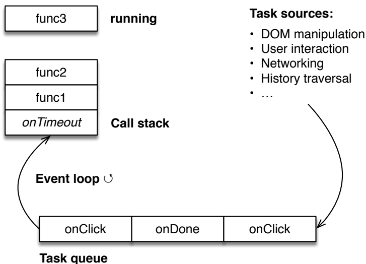
Figure 39.1: Task sources add code to run to the task queue , which is emptied by the event loop .
