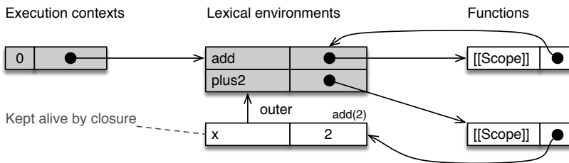
Figure 26.8: Closures, pause 2 – after the execution of add(2) : plus2 now points to the function returned by add(2) . That function keeps its birth environment (the environment of add(2) ) alive via its [[Scope]] .
