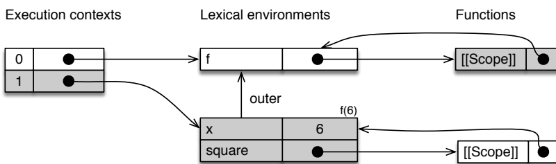
Figure 26.5: Nested scopes, pause 2 – while executing f() : There is now an environment for the function call f(6) . The outer environment of that environment is the birth environment of f() (the top-level environment at index 0). We can see that the field outer was set to the value of f 's [[Scope]] . Furthermore, the [[Scope]] of the new function square() is the environment that was just created.
