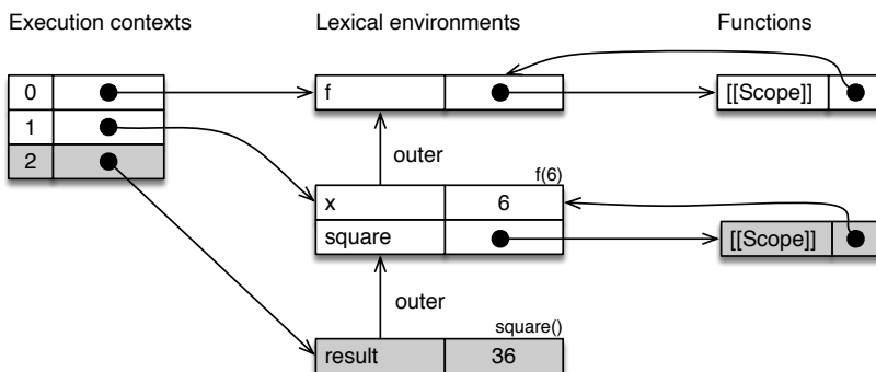
Figure 26.6: Nested scopes, pause 3 – while executing square() : The previous pattern was repeated: the outer of the most recent environment was set up via the [[Scope]] of the function that we just called. The chain of scopes created via outer , contains all variables that are active right now. For example, we can access result , square , and f if we want to. Environments reflect two aspects of variables. First, the chain of outer environments reflects the nested static scopes. Second, the stack of execution contexts reflects what function calls were made, dynamically.
