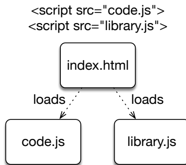
Figure 46.1: A classic, very simple web app: An HTML file refers to a JavaScript file code.js , which imbues the former with interactivity. code.js uses the library library.js , which must also be loaded by the HTML file.
