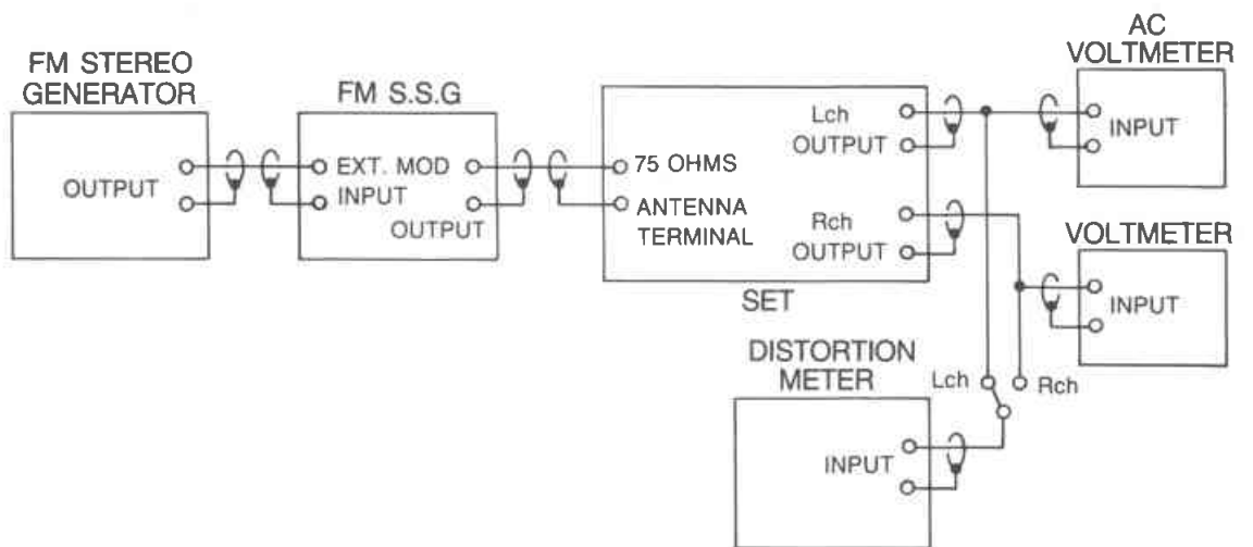
Fig. 4-2 Instrument connection for FM section adjustment
