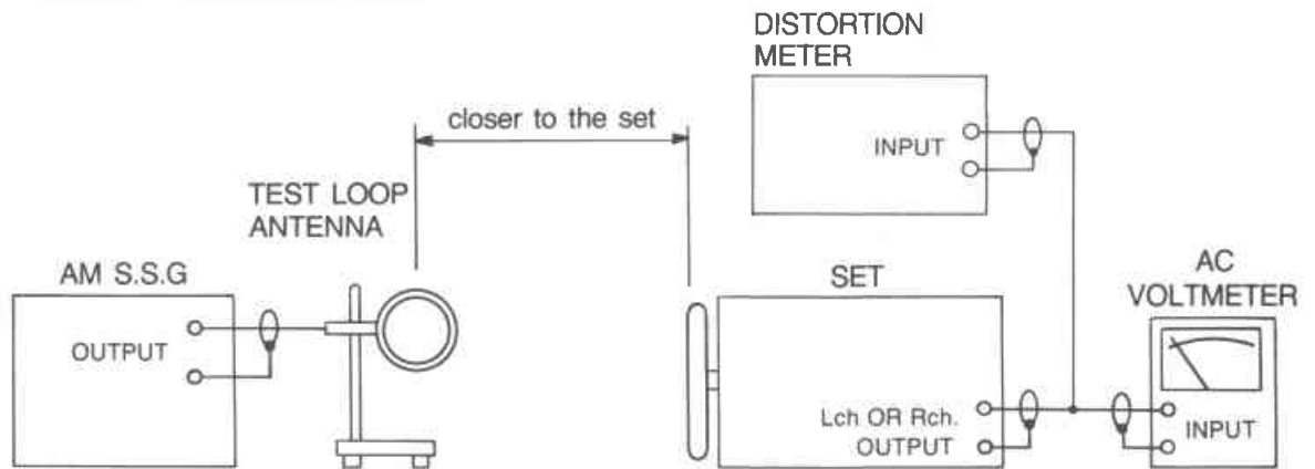
Fig. 4-1 Instrument connection for AM (MW, LW) section adjustment
